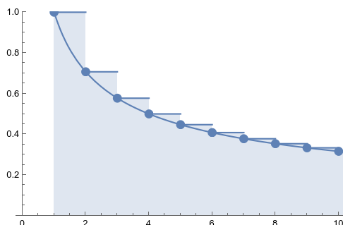
Figure 1.5: The series \sum \frac{1}{\sqrt{n}} diverges, because \int_1^\infty \frac{1}{\sqrt{x}} dx diverges.
