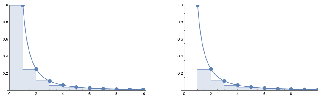
Figure 1.4: Removing the first rectangle changes the value of the integral, but can't affect whether it's finite or infinite.
