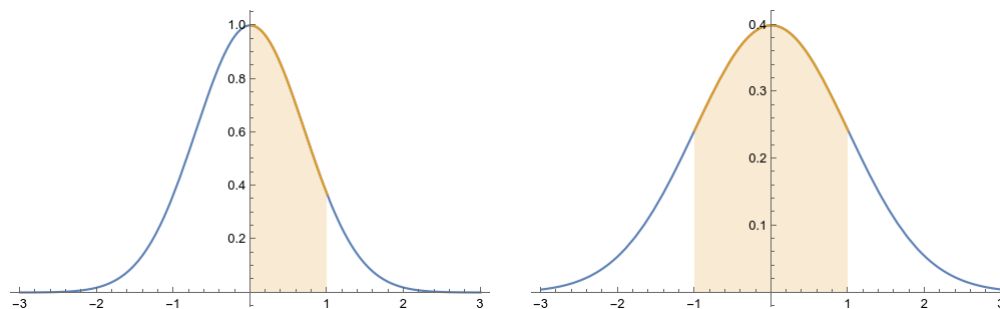
Figure 5.12: Left: \int_0^1 e^{-x^2} dx . Right: The probability of landing within one standard deviation of the mean.
